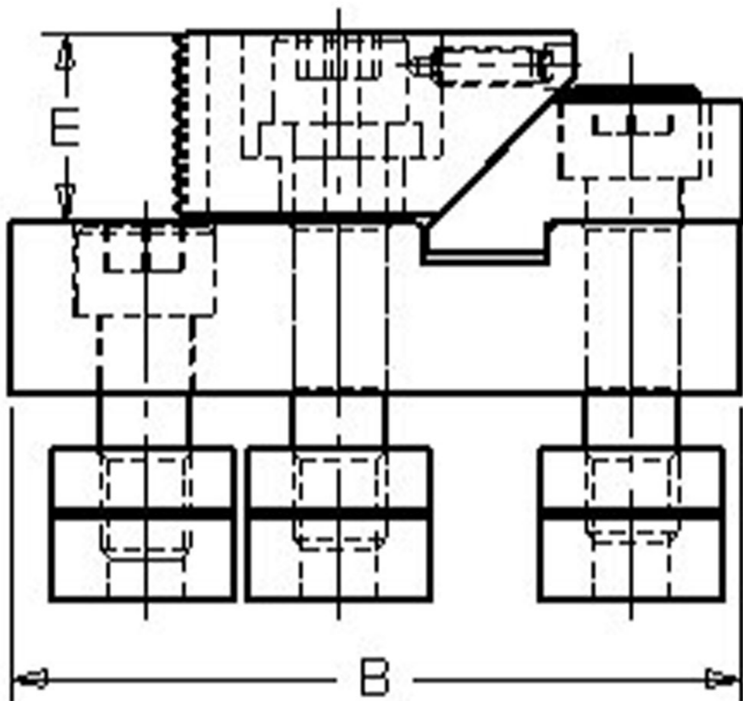
ADJUSTABLE JAW 46721
