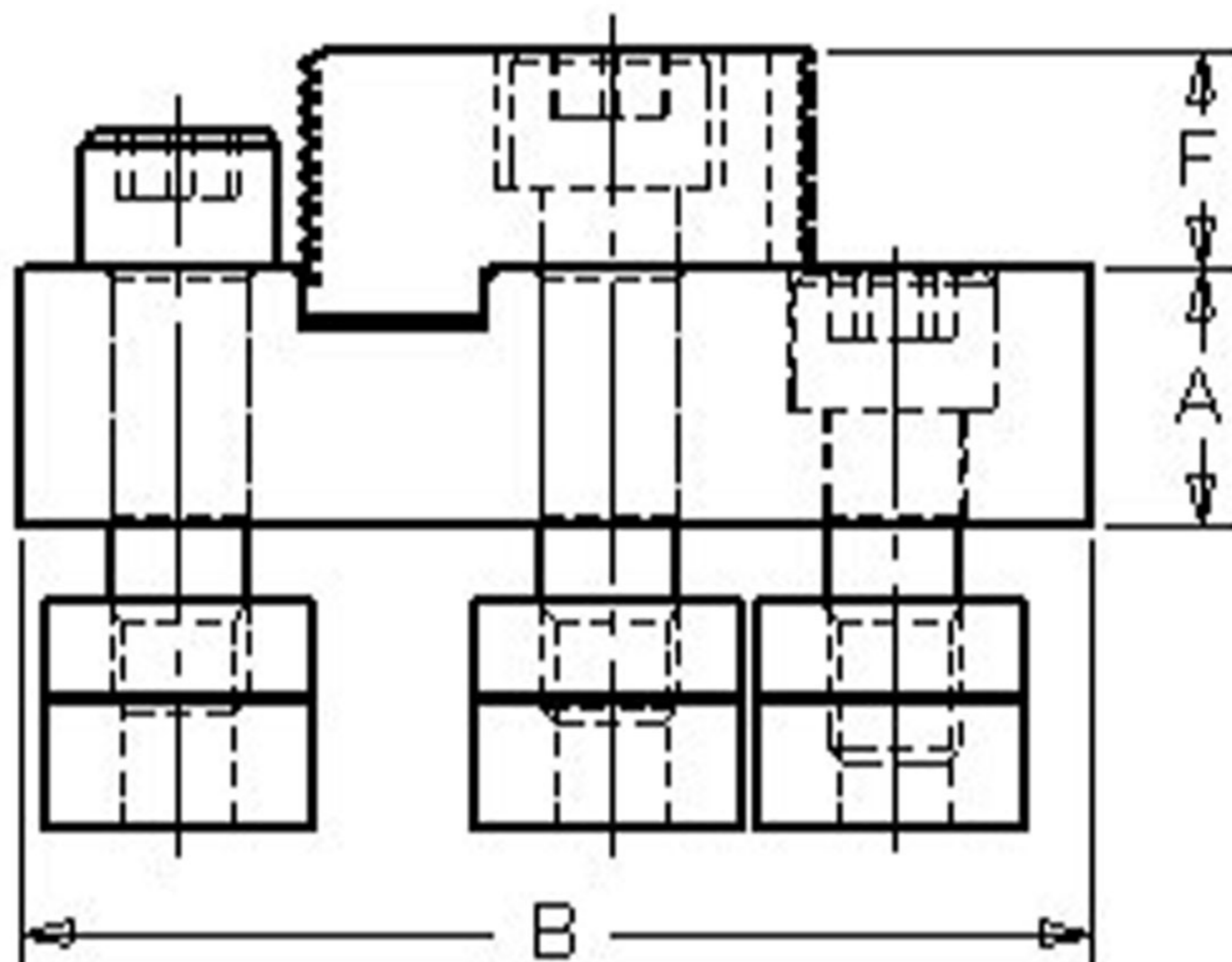
FIXED JAW 46711
