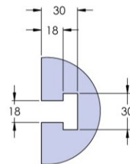
T-SLOT DETAIL A
