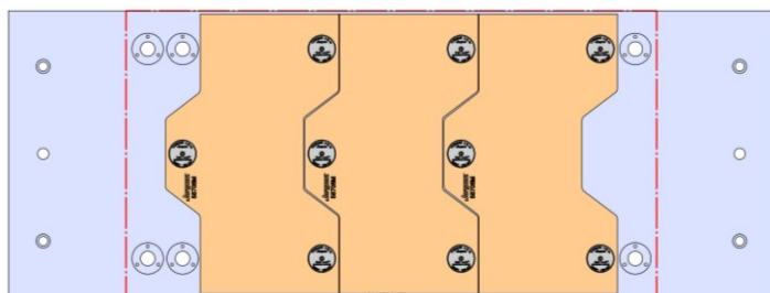
58706 Aluminum
