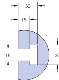
T-SLOT DETAIL A
