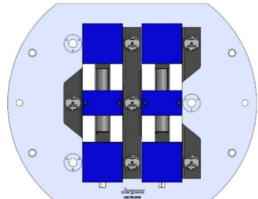
69405 100MM Vise Ball-Lock® Base
